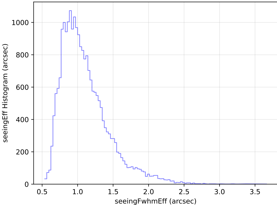
too_10_1v3.4_10yrs Yr 1 g band: seeingEff Histogram
