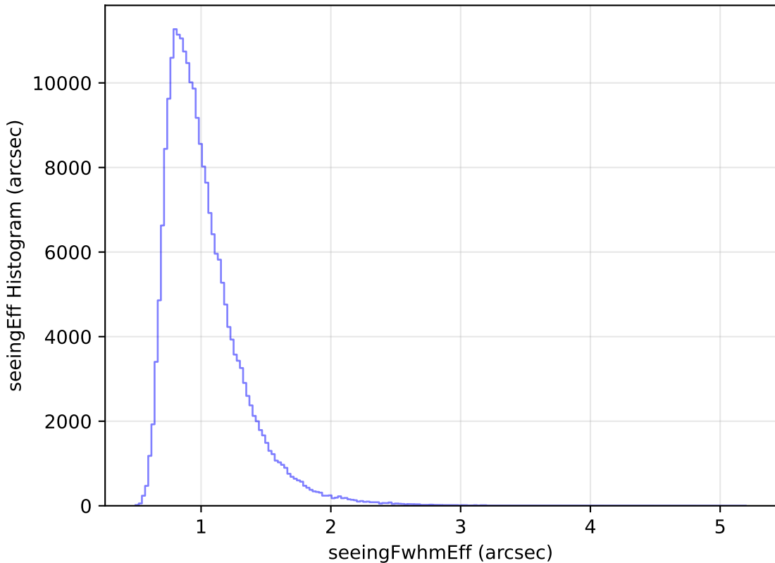
too_10_1v3.4_10yrs Yr 1 all bands: seeingEff Histogram
