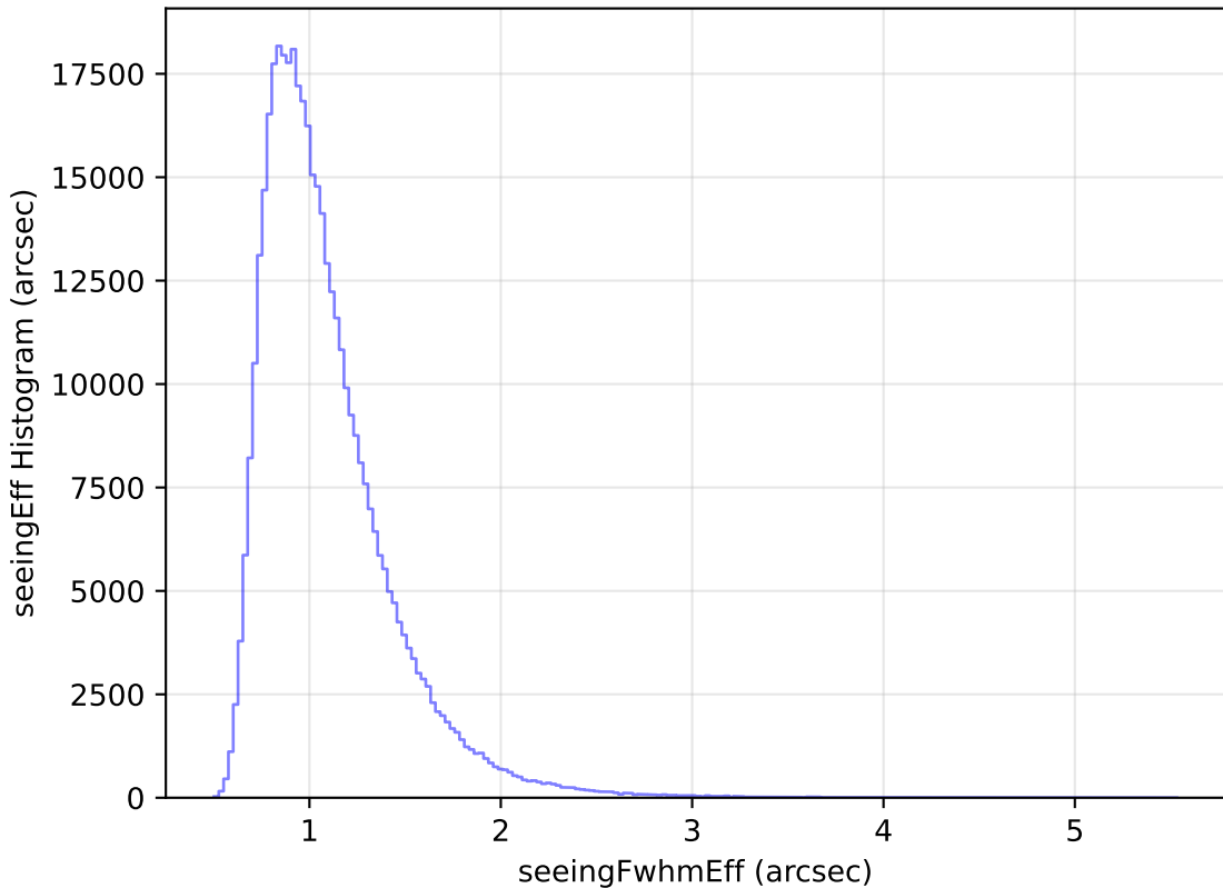
too_10_1v3.4_10yrs WFD z band: seeingEff Histogram
