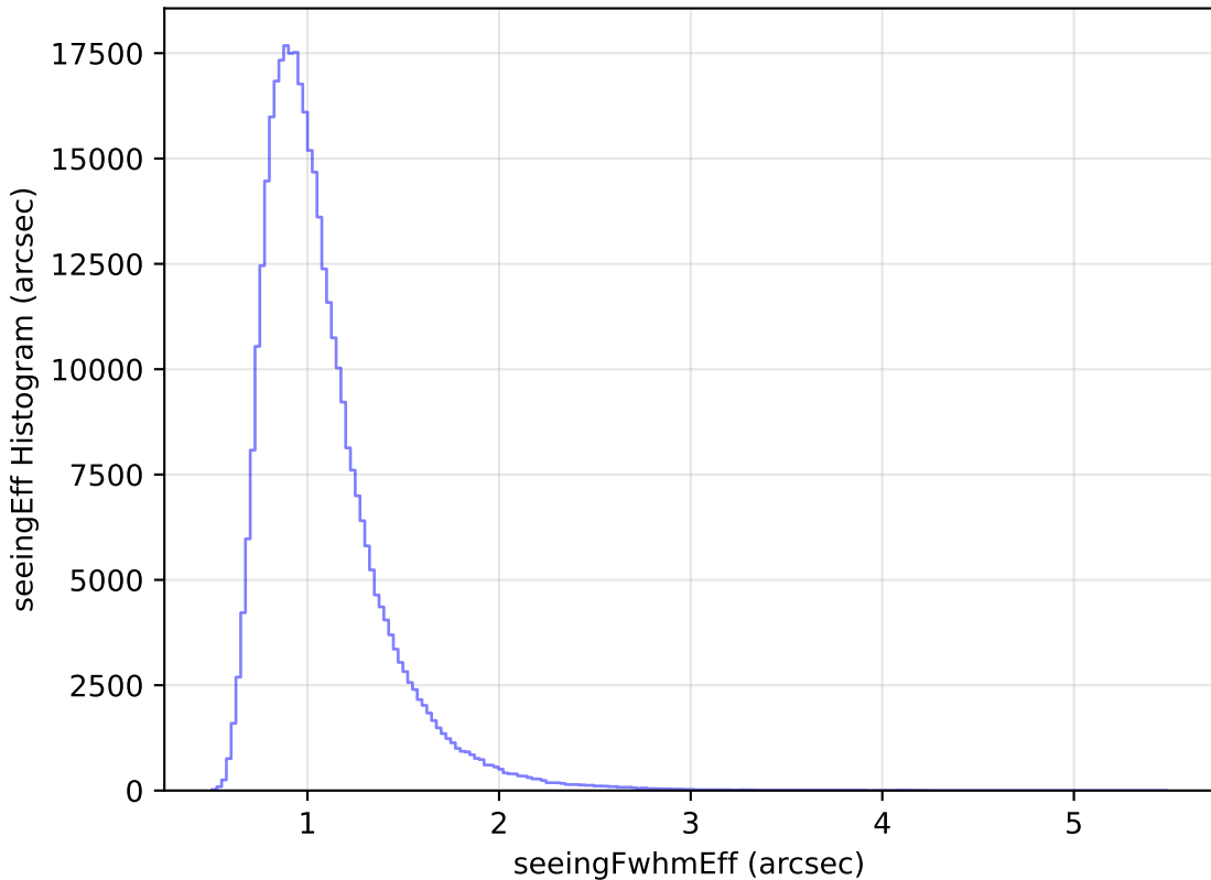
too_10_1v3.4_10yrs WFD y band: seeingEff Histogram
