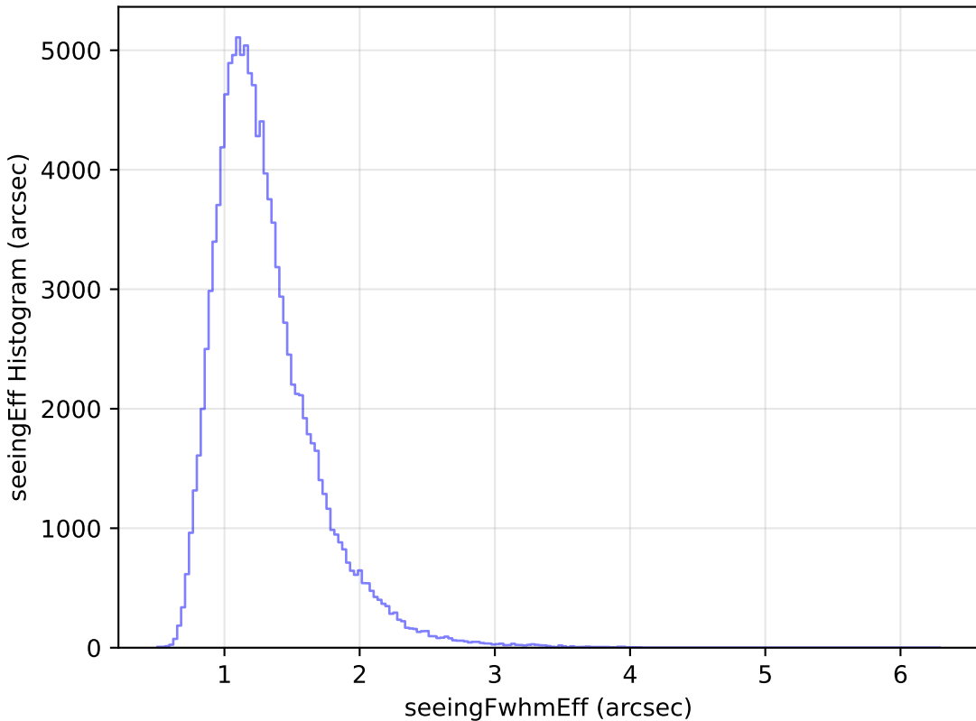
too_10_1v3.4_10yrs WFD u band: seeingEff Histogram
