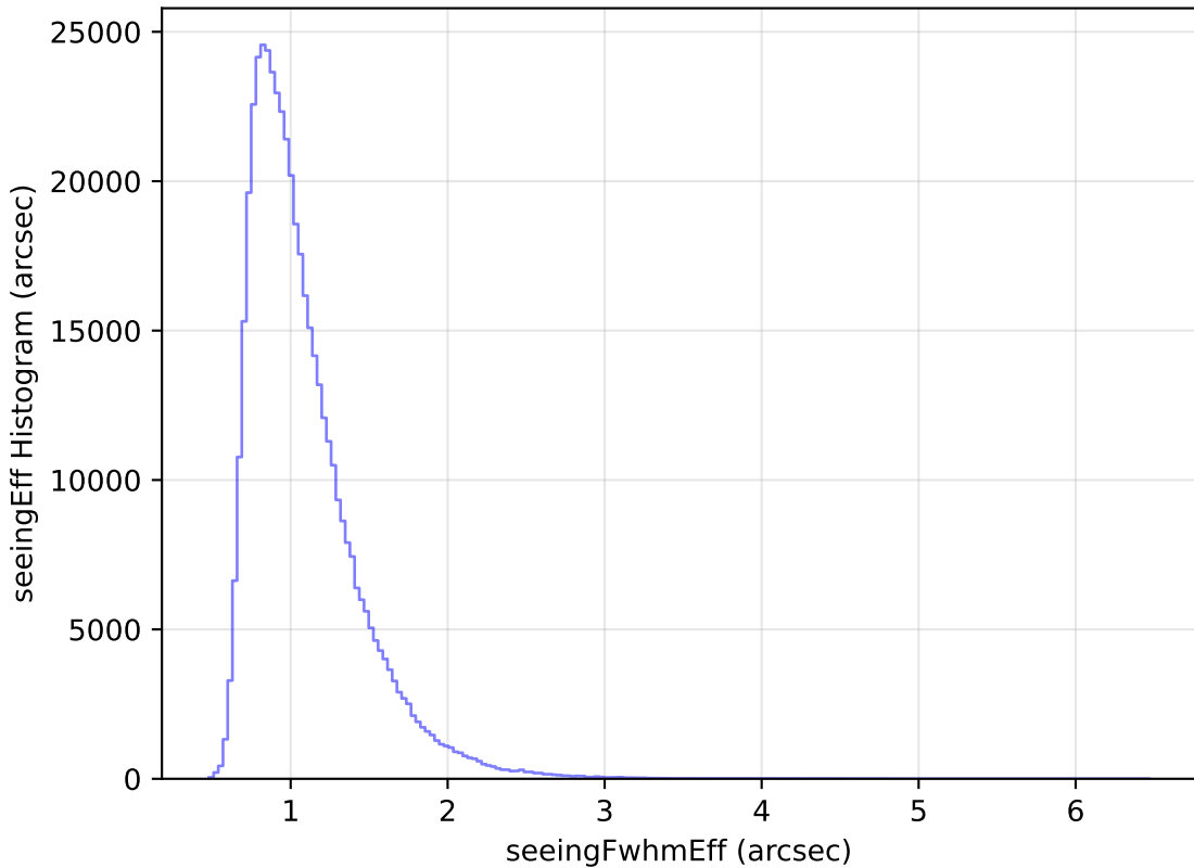
too_10_1v3.4_10yrs WFD i band: seeingEff Histogram
