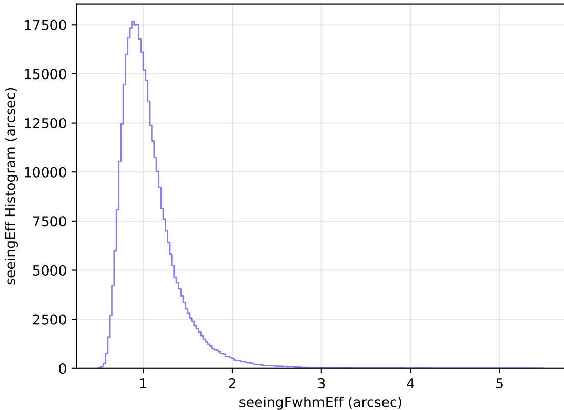
too_10_1v3.4_10yrs All sky y band: seeingEff Histogram
