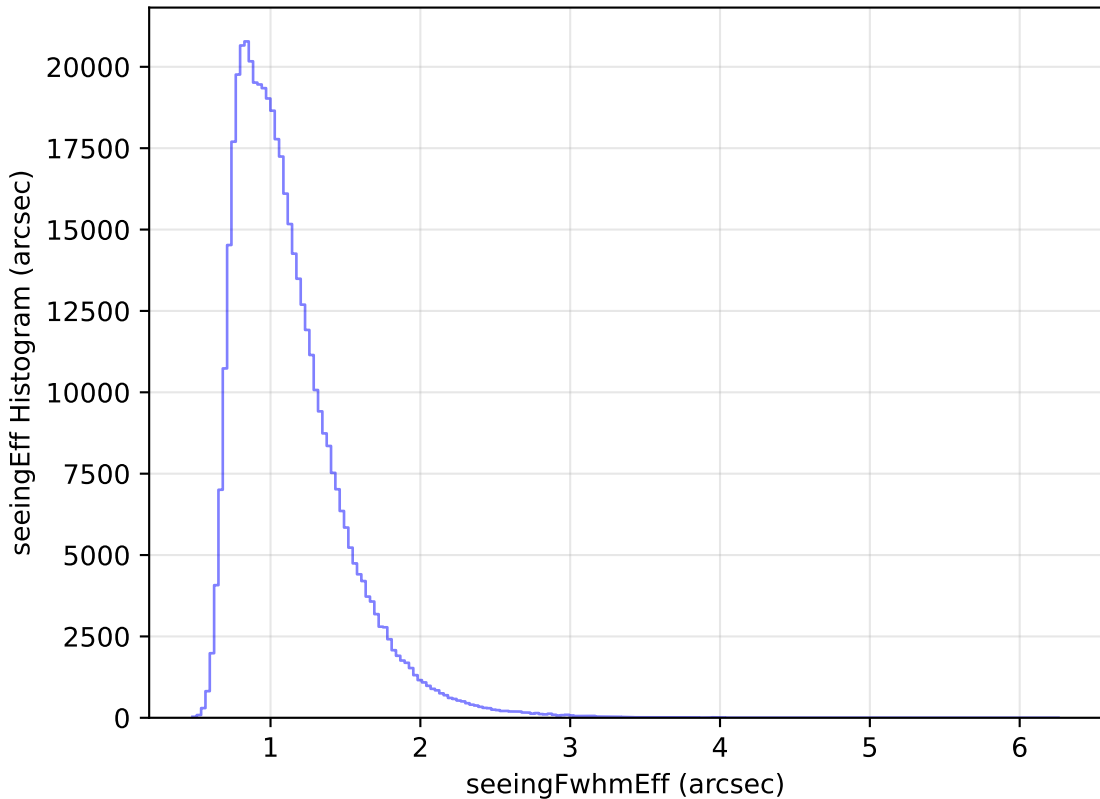
too_10_1v3.4_10yrs All sky r band: seeingEff Histogram
