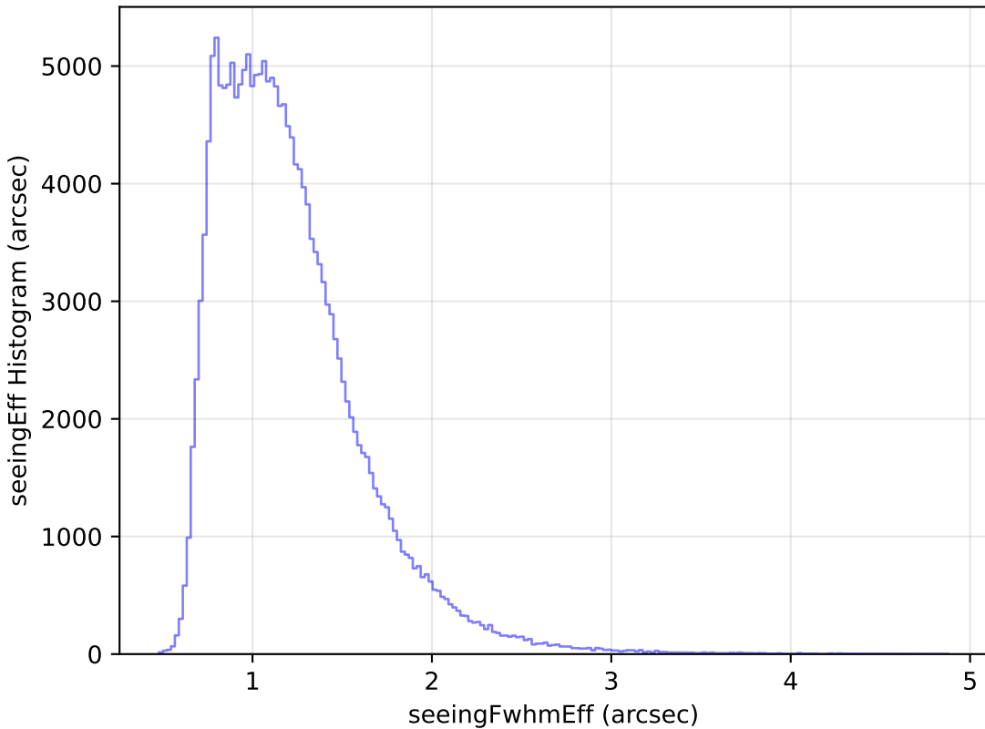
too_10_1v3.4_10yrs All sky g band: seeingEff Histogram
