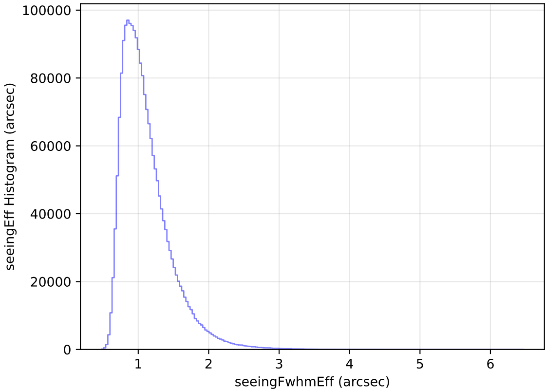
too_10_1v3.4_10yrs All sky all bands: seeingEff Histogram
