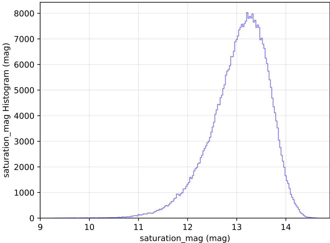
too_10_1v3.4_10yrs WFD y band: saturation_mag Histogram
