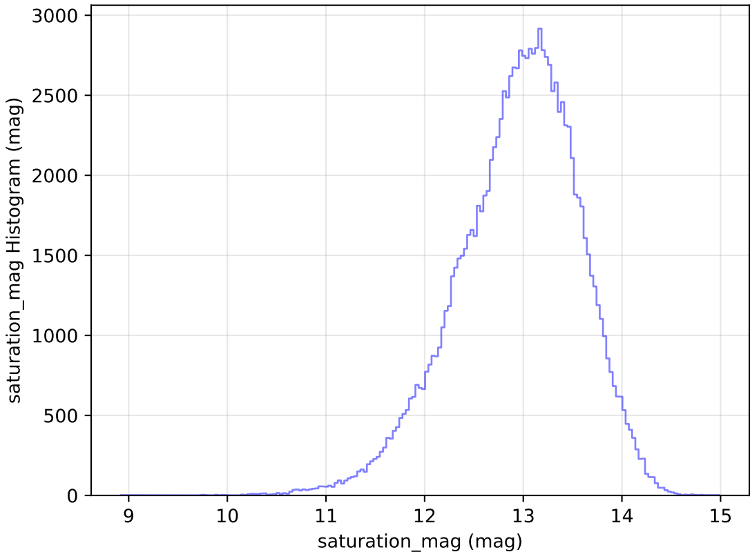
too_10_1v3.4_10yrs WFD u band: saturation_mag Histogram
