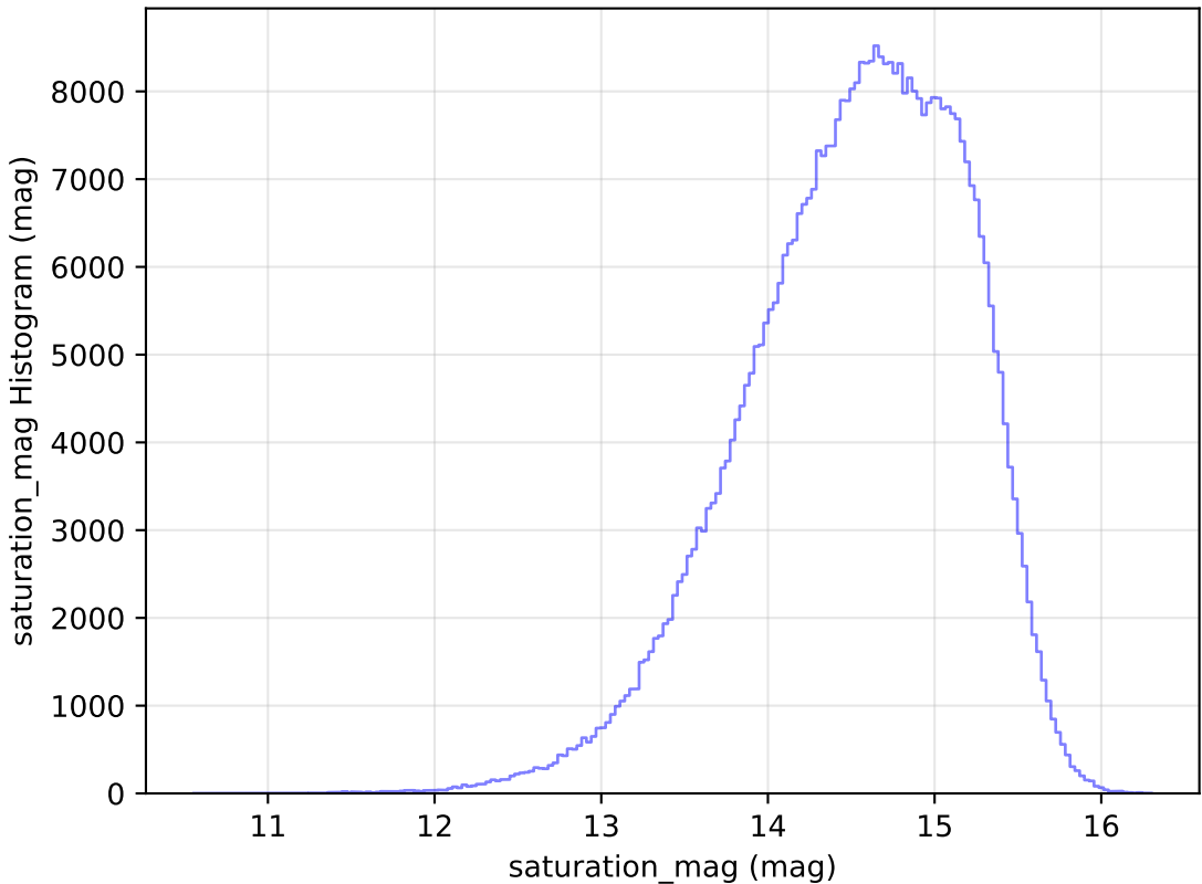
too_10_1v3.4_10yrs WFD r band: saturation_mag Histogram
