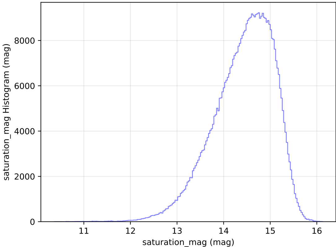
too_10_1v3.4_10yrs WFD i band: saturation_mag Histogram
