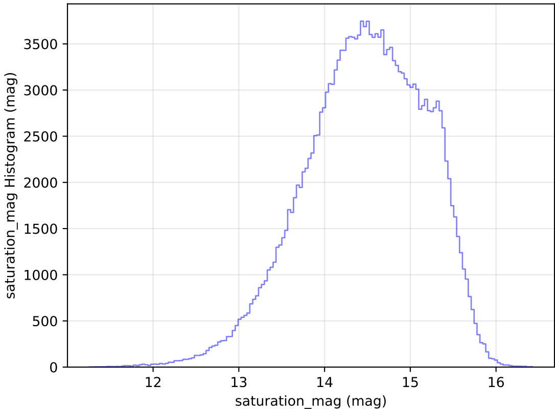
too_10_1v3.4_10yrs WFD g band: saturation_mag Histogram
