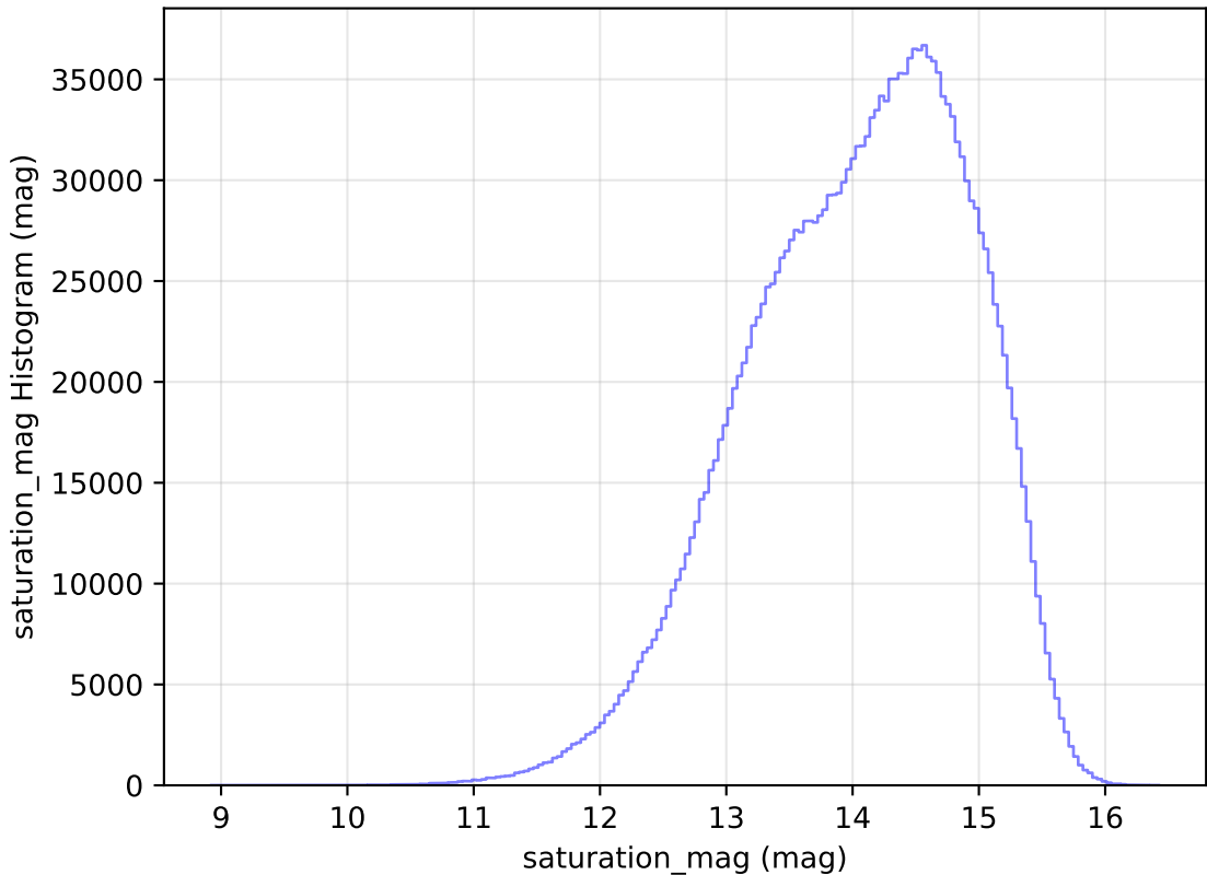
too_10_1v3.4_10yrs WFD all bands: saturation_mag Histogram
