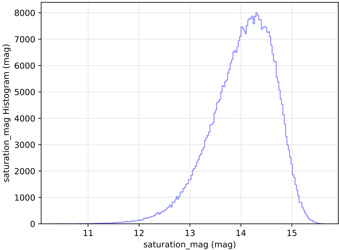
too_10_1v3.4_10yrs All sky z band: saturation_mag Histogram
