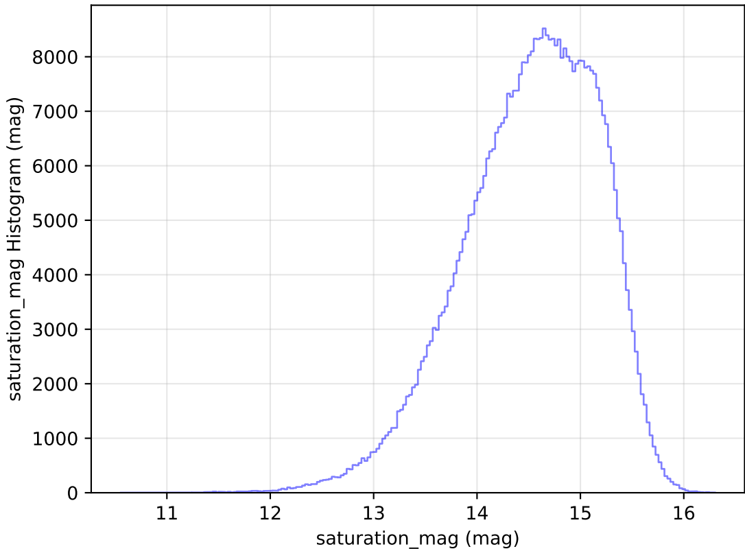
too_10_1v3.4_10yrs All sky r band: saturation_mag Histogram
