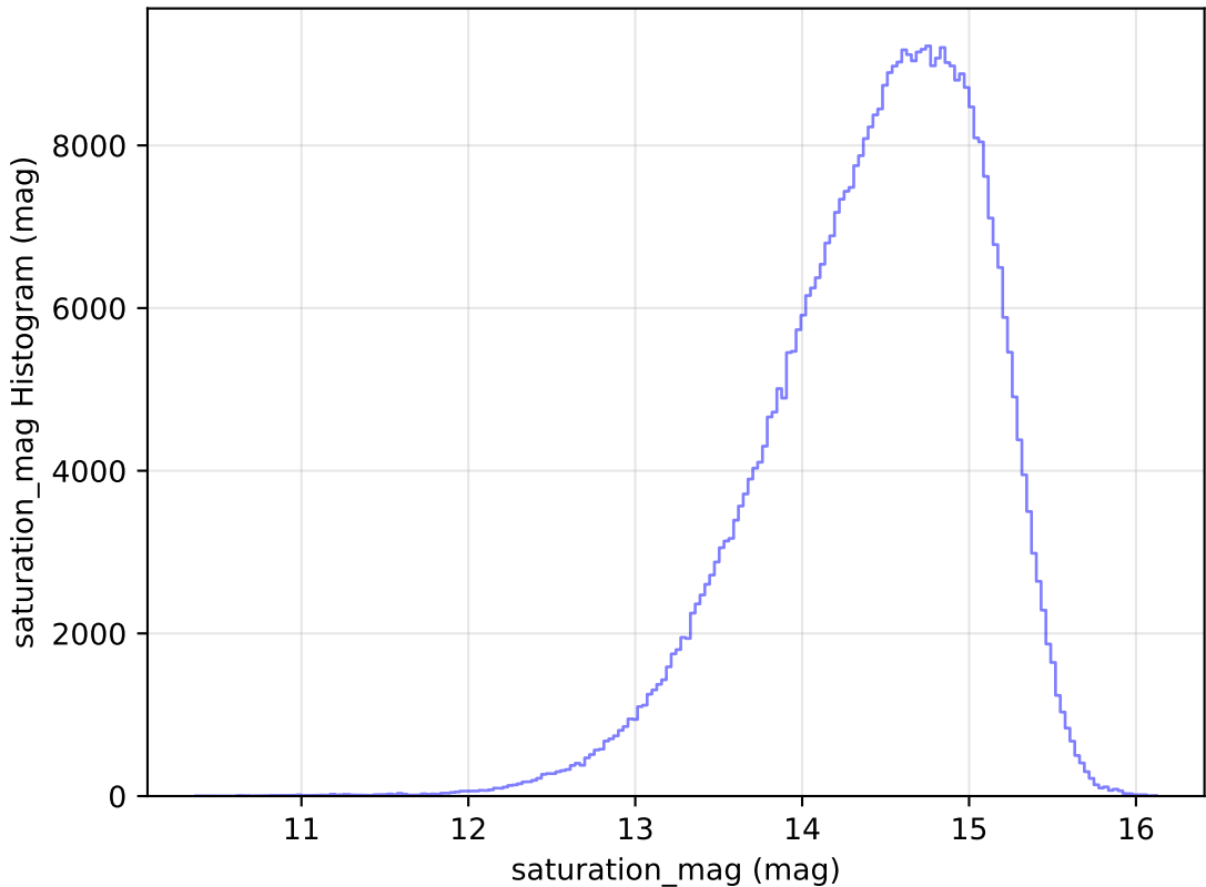
too_10_1v3.4_10yrs All sky i band: saturation_mag Histogram
