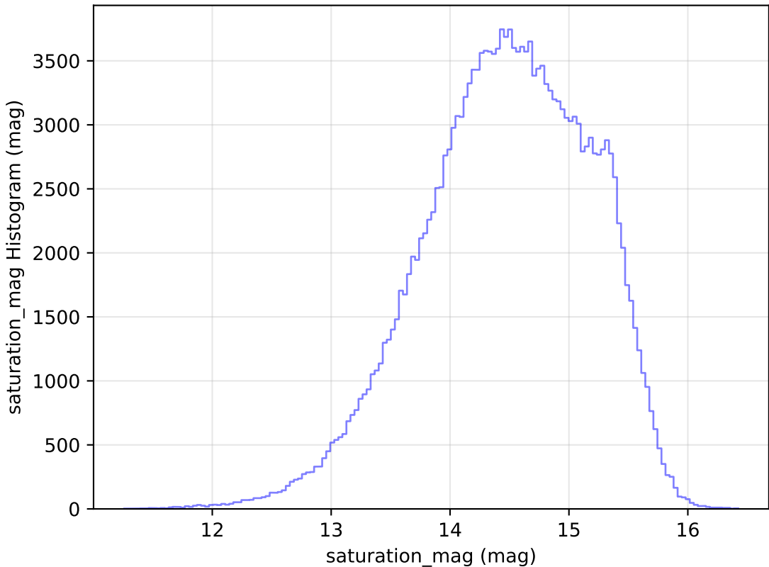
too_10_1v3.4_10yrs All sky g band: saturation_mag Histogram
