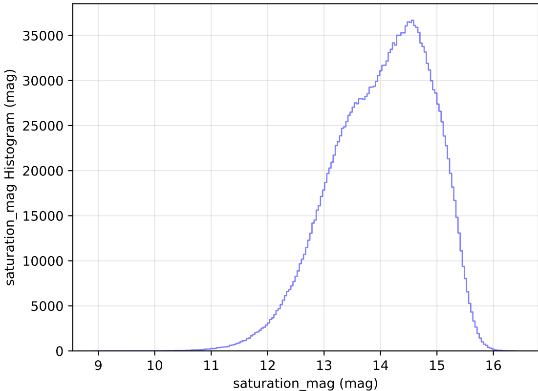
too_10_1v3.4_10yrs All sky all bands: saturation_mag Histogram
