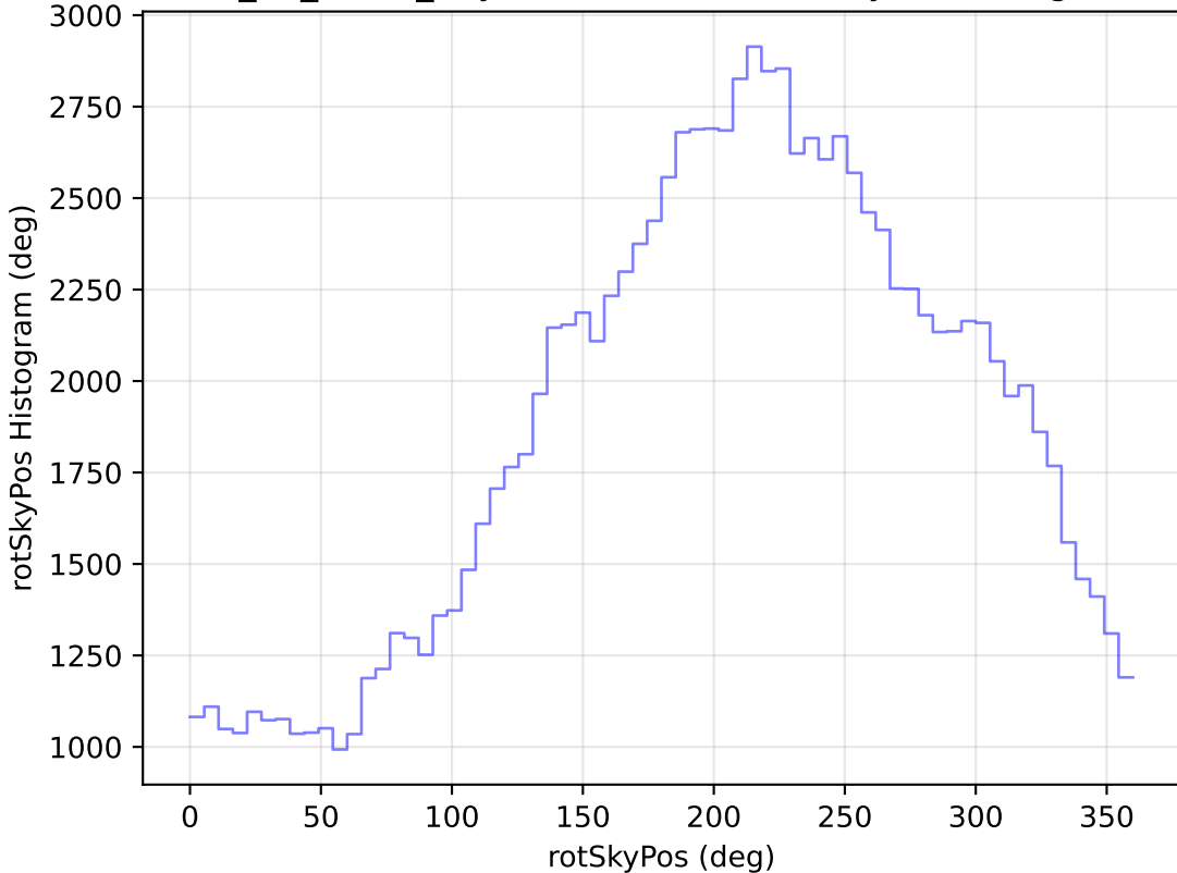
too_10_1v3.4_10yrs WFD u band: rotSkyPos Histogram
