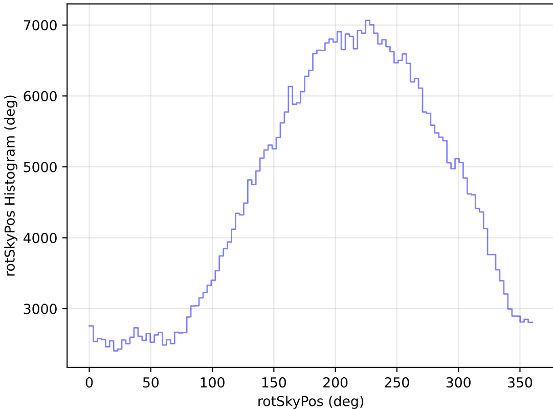
too_10_1v3.4_10yrs WFD i band: rotSkyPos Histogram
