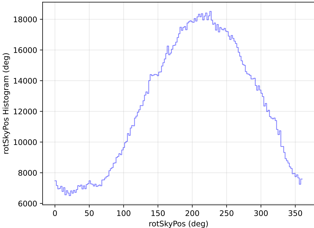
too_10_1v3.4_10yrs WFD all bands: rotSkyPos Histogram
