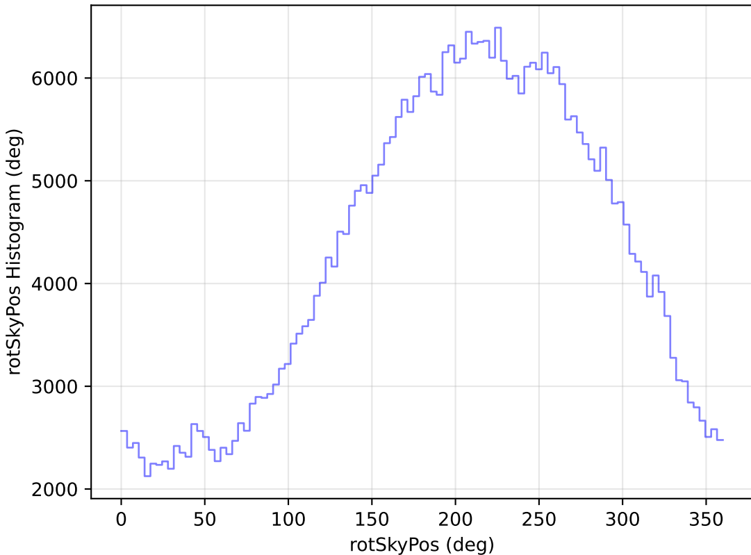
too_10_1v3.4_10yrs All sky z band: rotSkyPos Histogram
