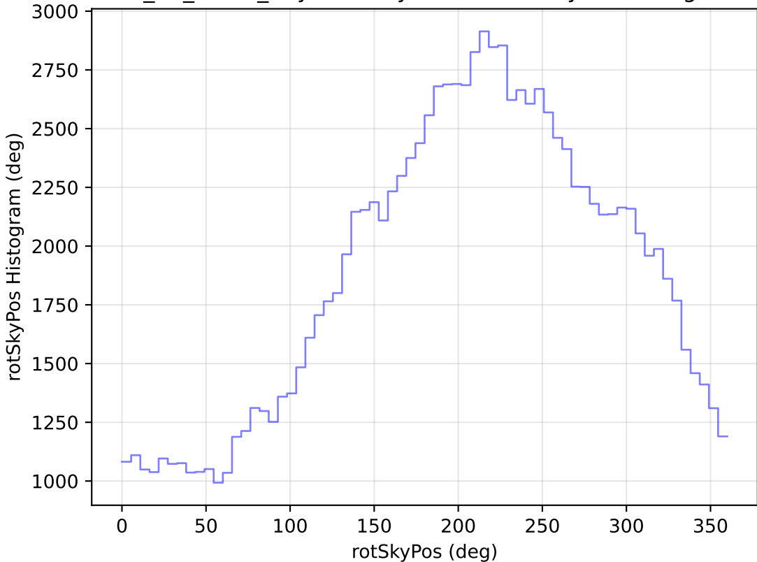
too_10_1v3.4_10yrs All sky u band: rotSkyPos Histogram
