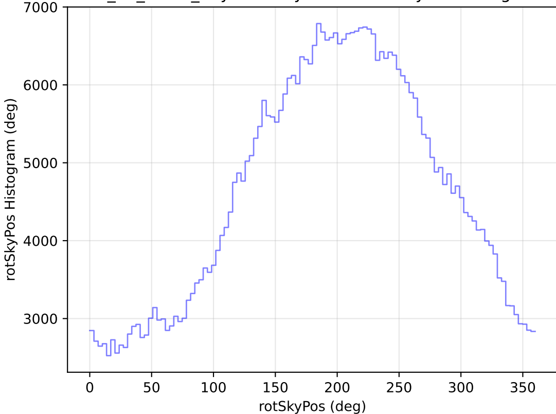
too_10_1v3.4_10yrs All sky r band: rotSkyPos Histogram
