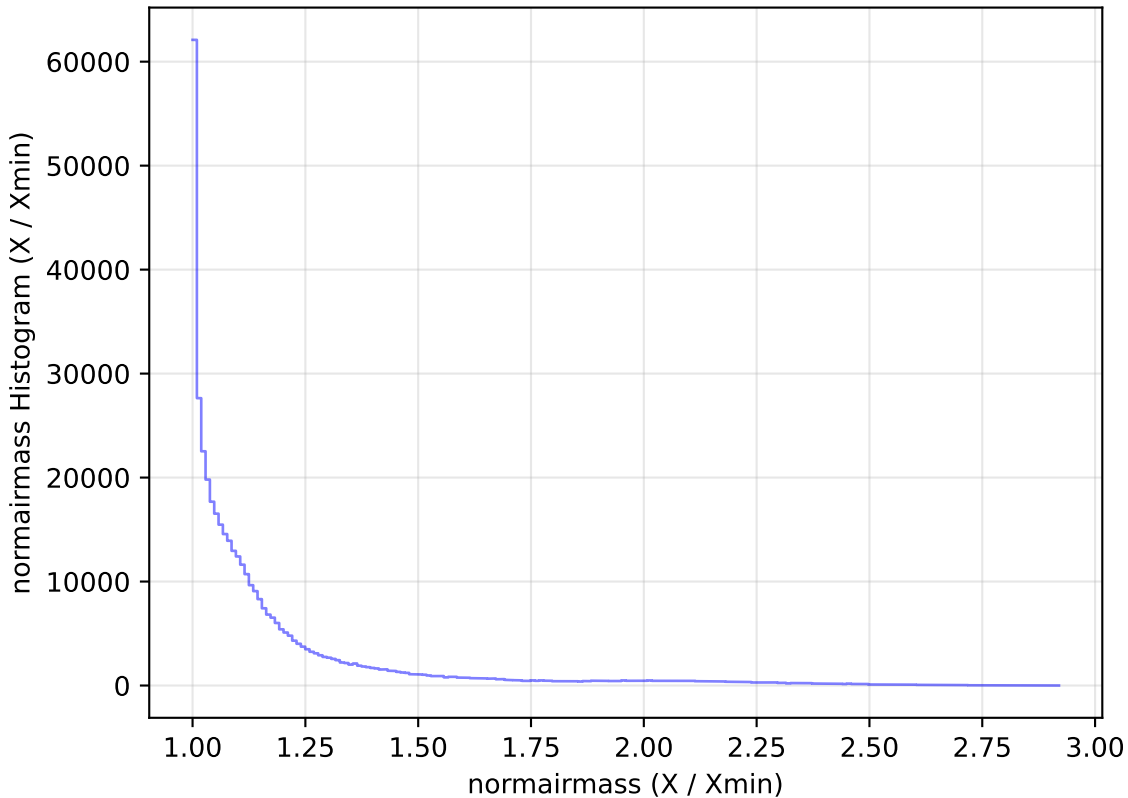
too_10_1v3.4_10yrs WFD z band: normairmass Histogram
