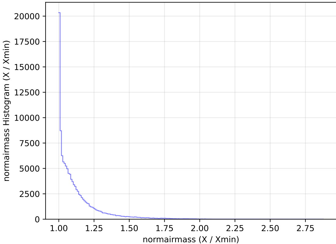
too_10_1v3.4_10yrs WFD u band: normairmass Histogram
