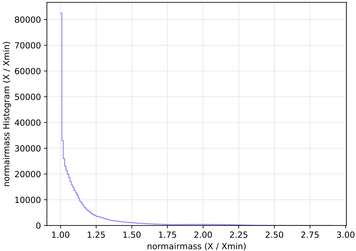
too_10_1v3.4_10yrs WFD r band: normairmass Histogram
