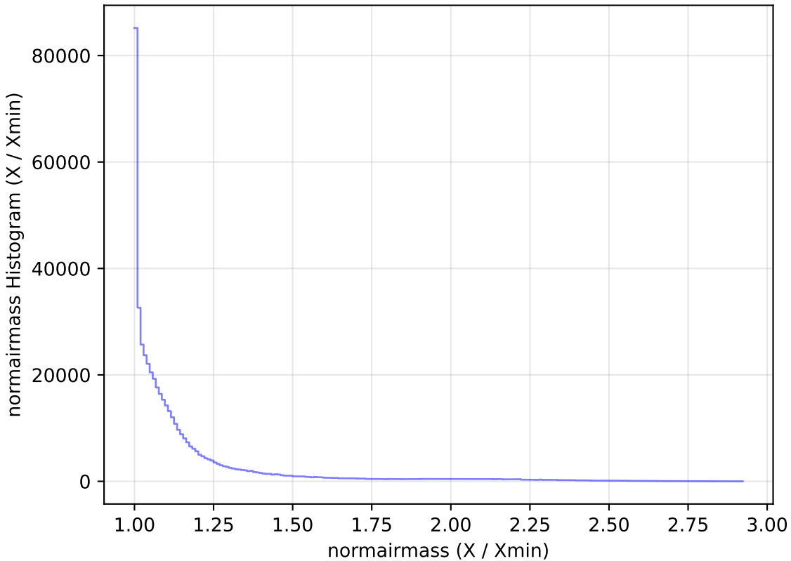
too_10_1v3.4_10yrs WFD i band: normairmass Histogram
