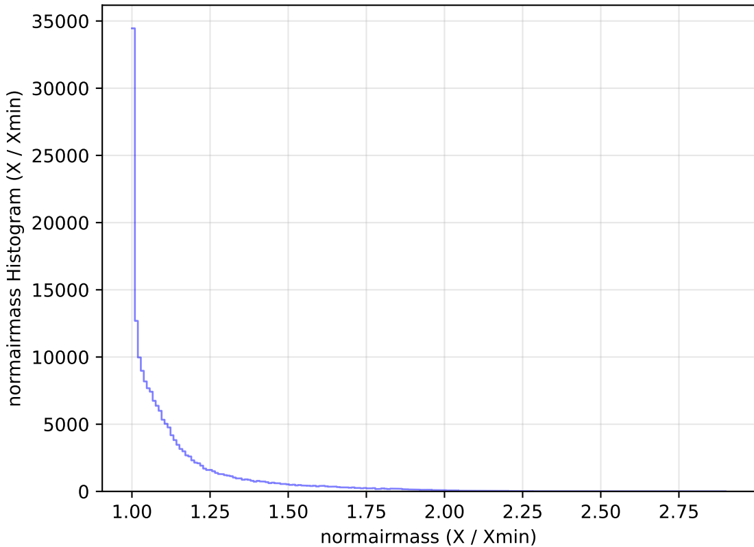
too_10_1v3.4_10yrs WFD g band: normairmass Histogram
