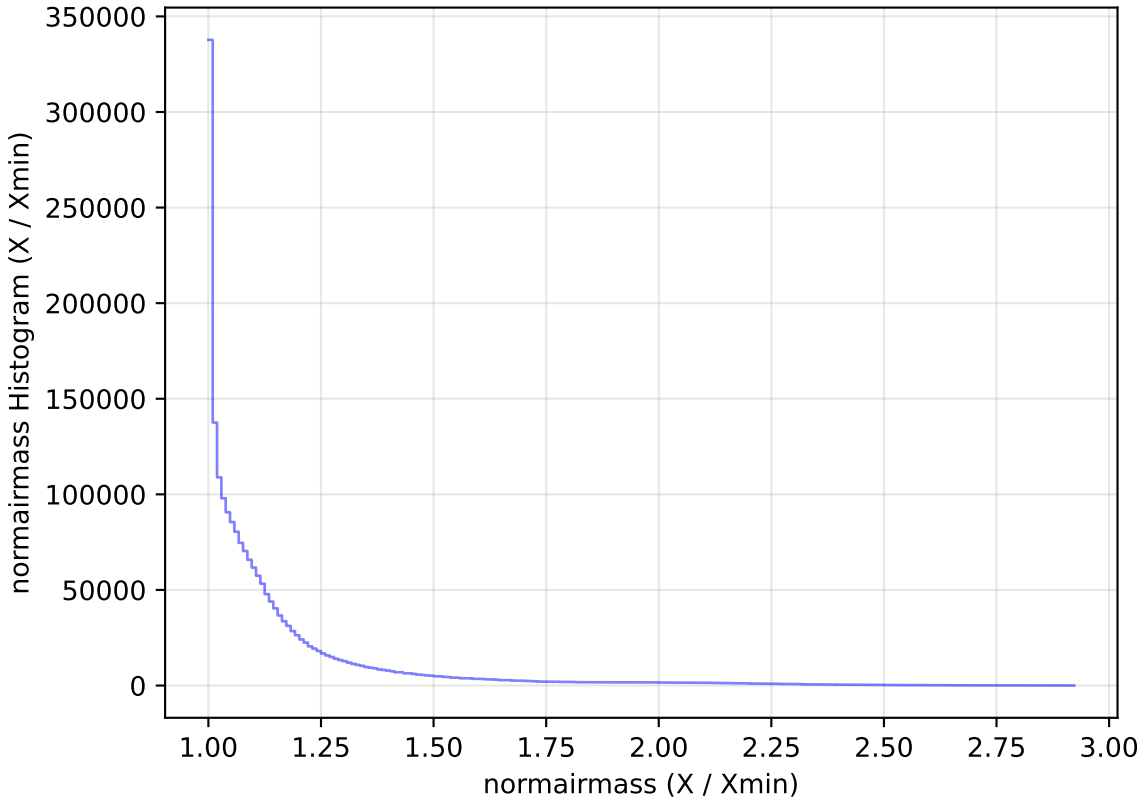
too_10_1v3.4_10yrs WFD all bands: normairmass Histogram
