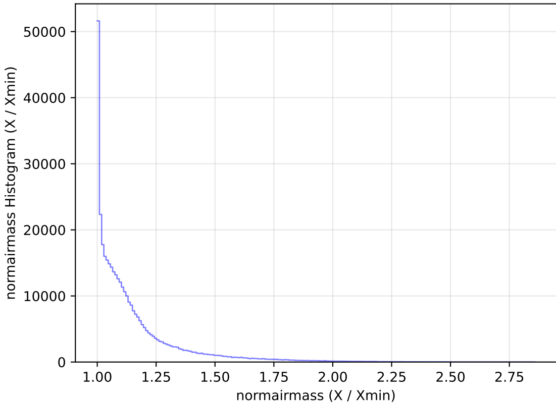
too_10_1v3.4_10yrs All sky y band: normairmass Histogram
