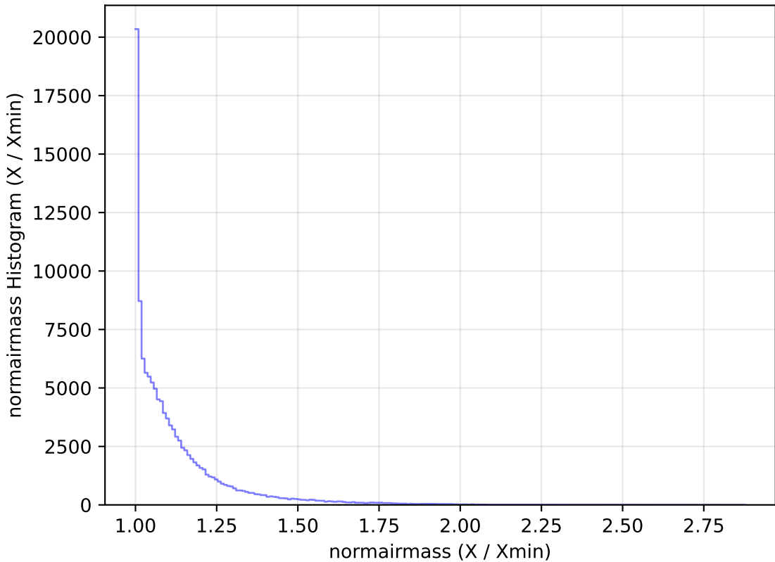
too_10_1v3.4_10yrs All sky u band: normairmass Histogram
