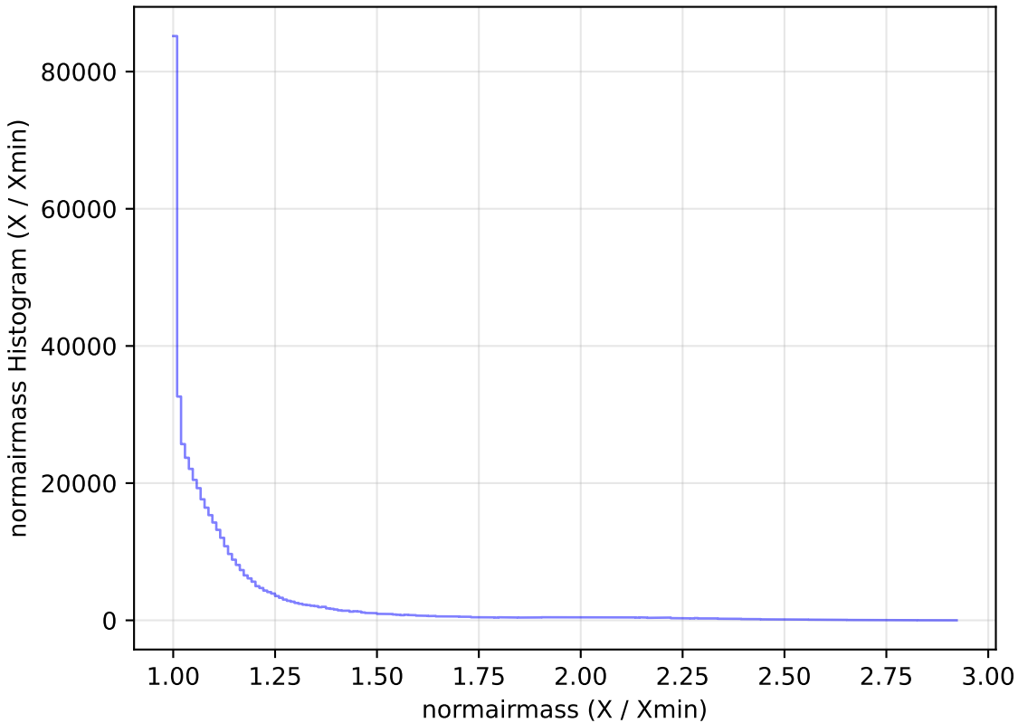
too_10_1v3.4_10yrs All sky i band: normairmass Histogram
