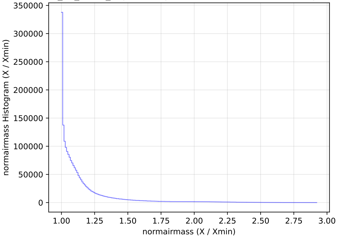
too_10_1v3.4_10yrs All sky all bands: normairmass Histogram
