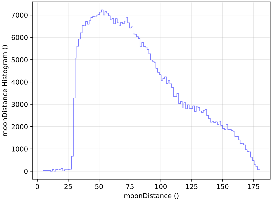
too_10_1v3.4_10yrs WFD z band: moonDistance Histogram
