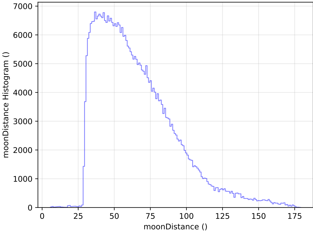
too_10_1v3.4_10yrs WFD y band: moonDistance Histogram
