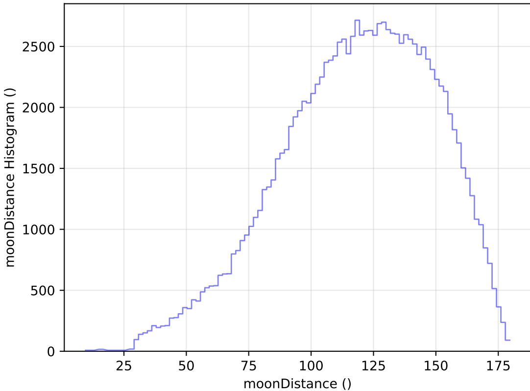
too_10_1v3.4_10yrs WFD u band: moonDistance Histogram
