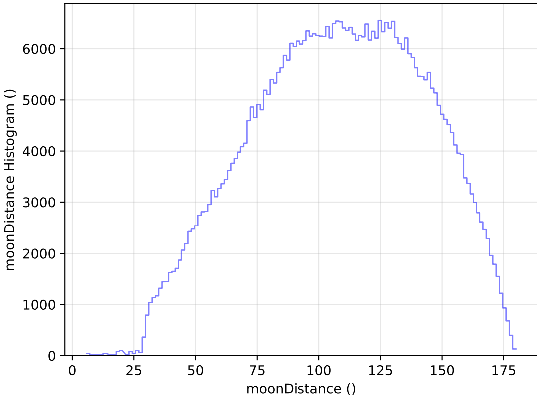
too_10_1v3.4_10yrs WFD r band: moonDistance Histogram
