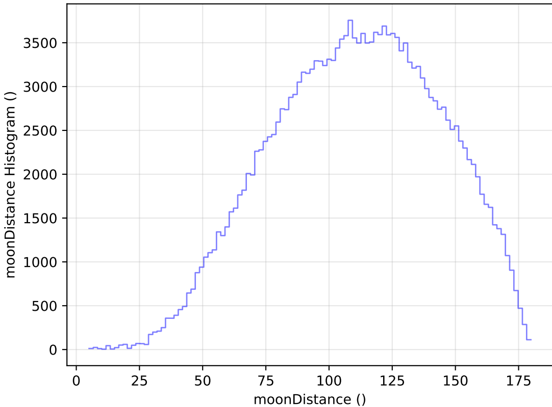
too_10_1v3.4_10yrs WFD g band: moonDistance Histogram
