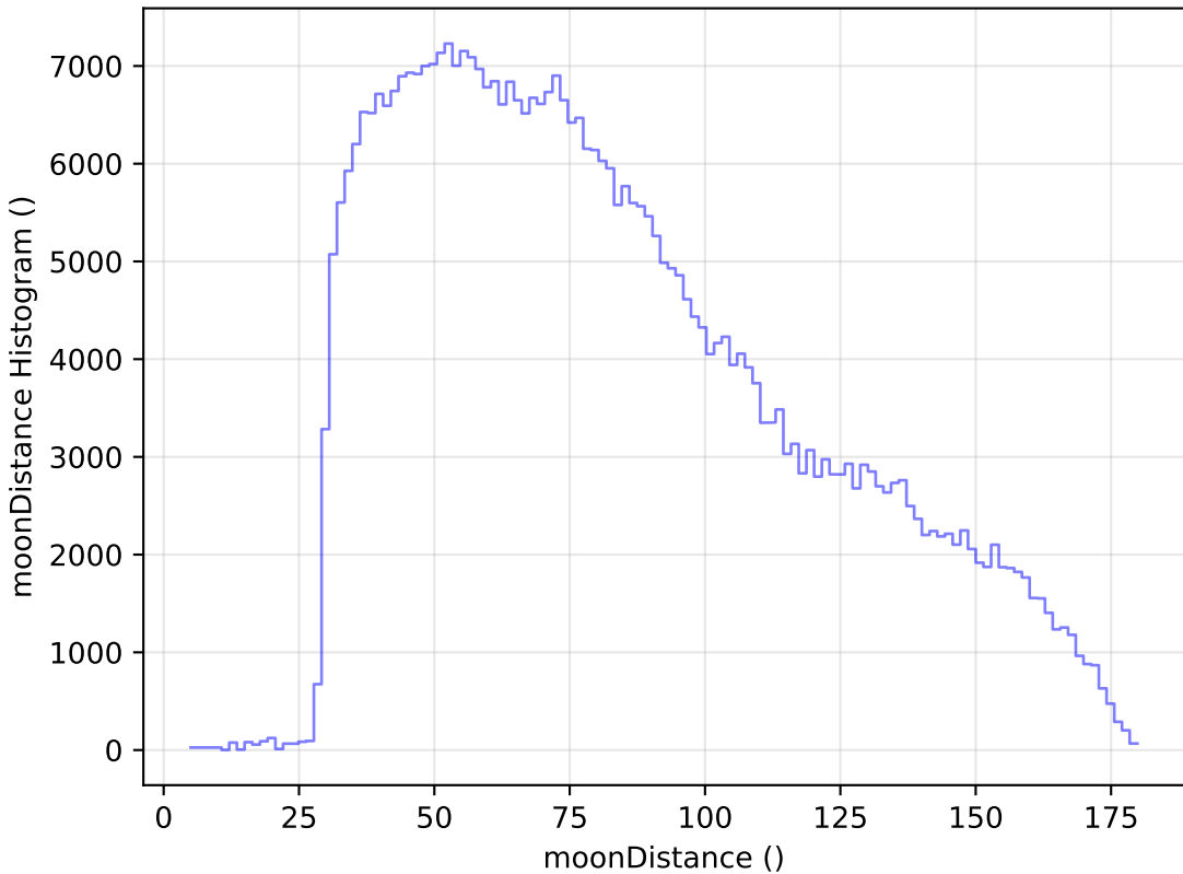
too_10_1v3.4_10yrs All sky z band: moonDistance Histogram
