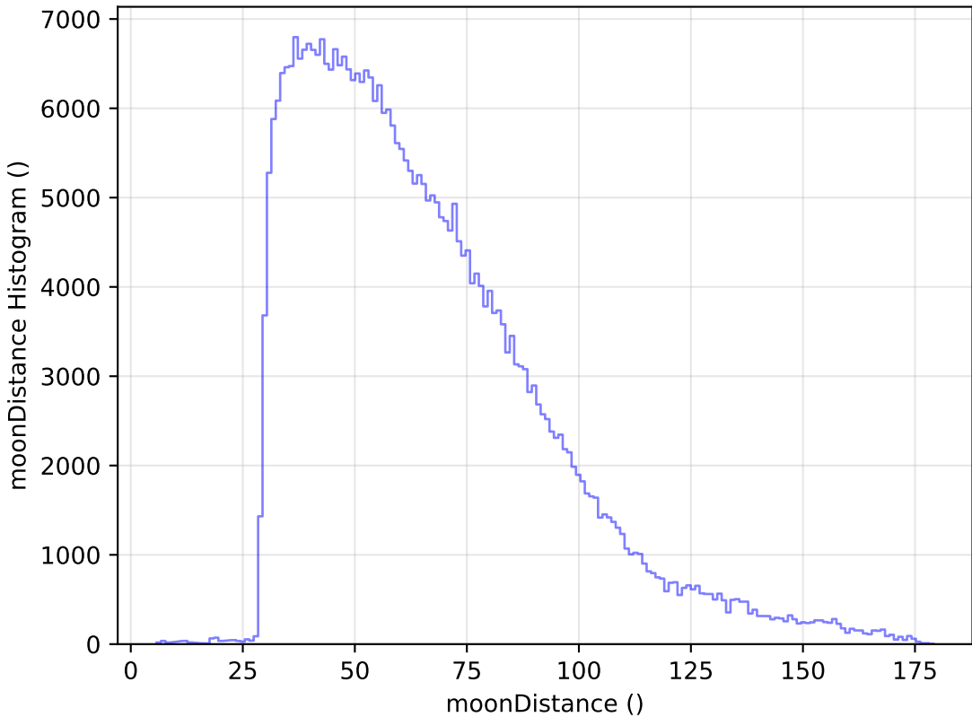
too_10_1v3.4_10yrs All sky y band: moonDistance Histogram
