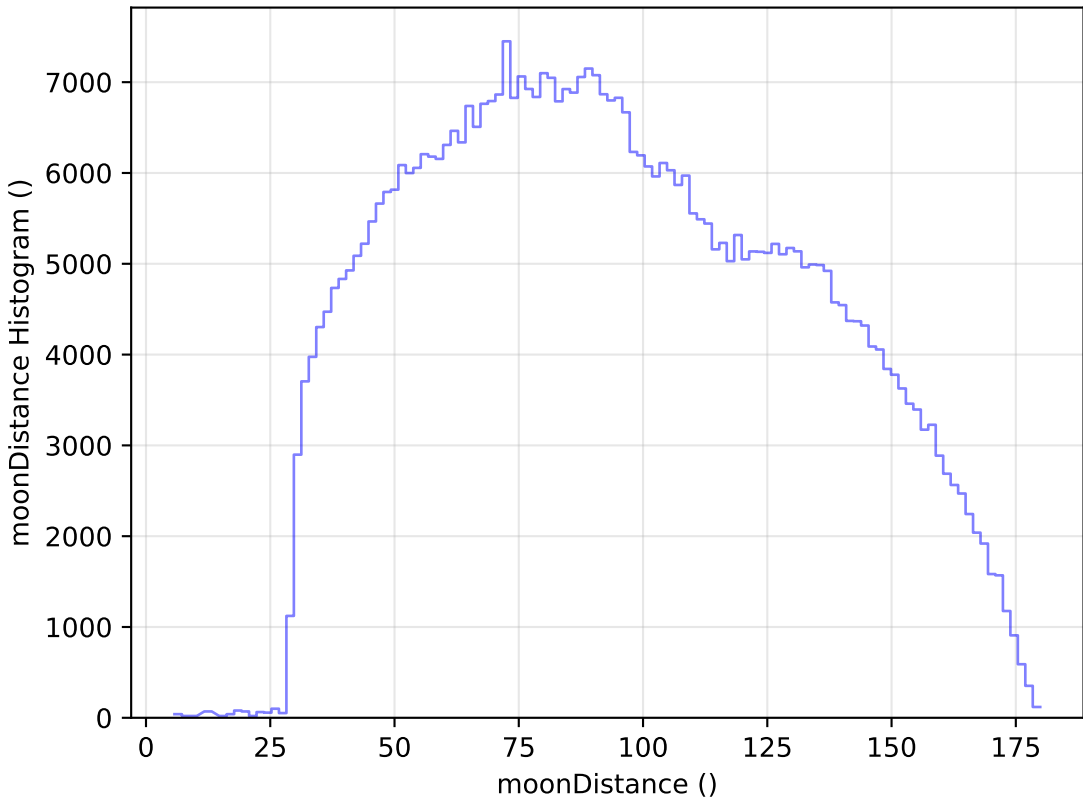
too_10_1v3.4_10yrs All sky i band: moonDistance Histogram
