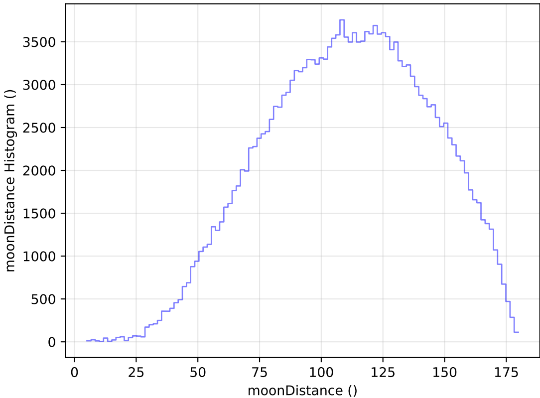
too_10_1v3.4_10yrs All sky g band: moonDistance Histogram
