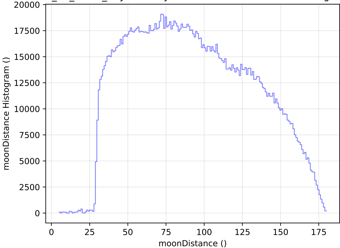
too_10_1v3.4_10yrs All sky all bands: moonDistance Histogram
