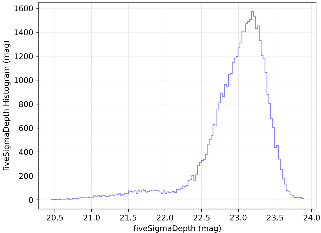
too_10_1v3.4_10yrs Yr 1 z band: fiveSigmaDepth Histogram
