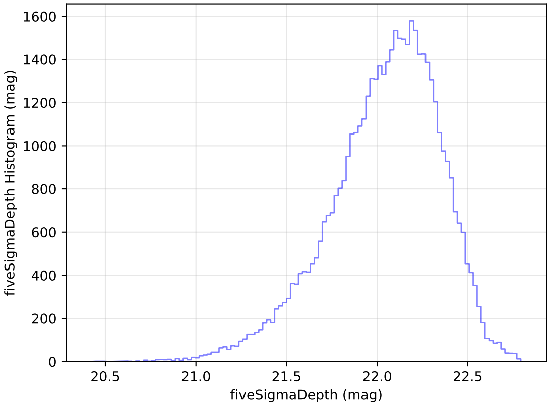
too_10_1v3.4_10yrs Yr 1 y band: fiveSigmaDepth Histogram
