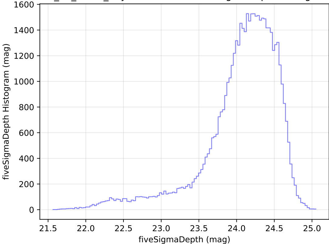
too_10_1v3.4_10yrs Yr 1 r band: fiveSigmaDepth Histogram
